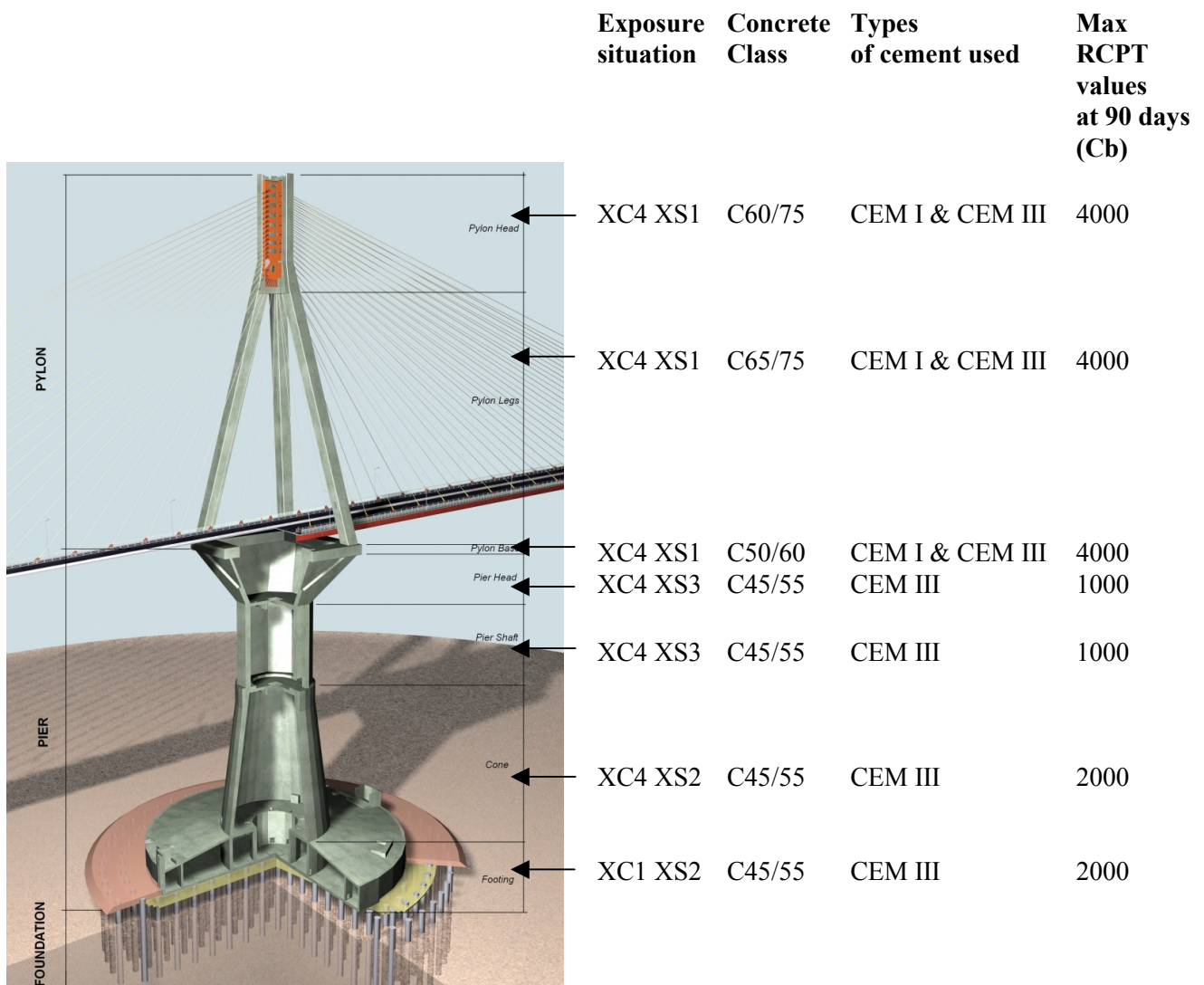
Figure 1. Main piers and pylons
